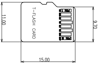
T-FLASH CARD PIN ASSIGNMENT
